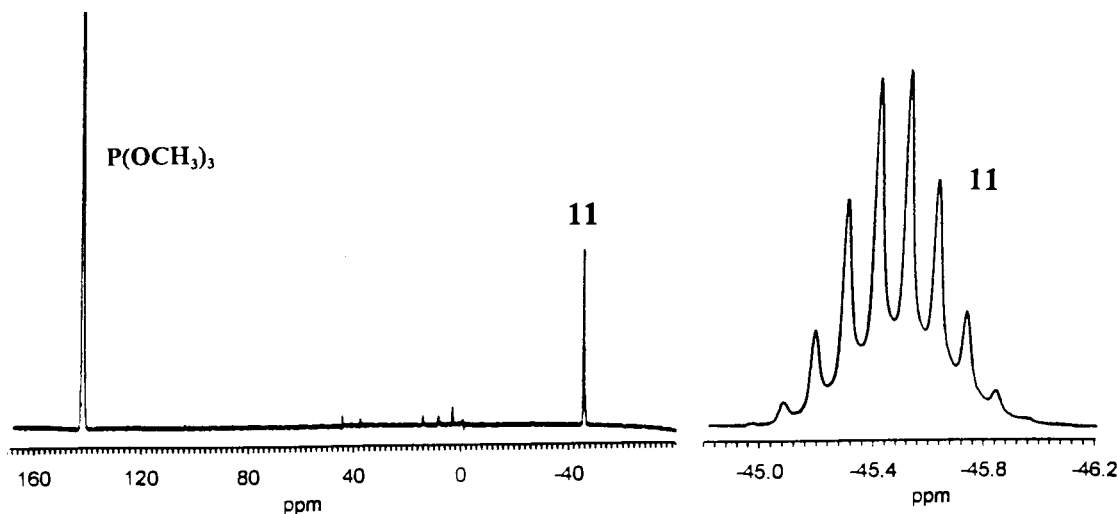
Figure 2. Reactions of o -benzoquinones with trimethyl phosphite and ^{31}\text{P} NMR spectra of compound 11 . Its proton-coupled spectrum gives eight well-resolved and two very weak lines (right).
